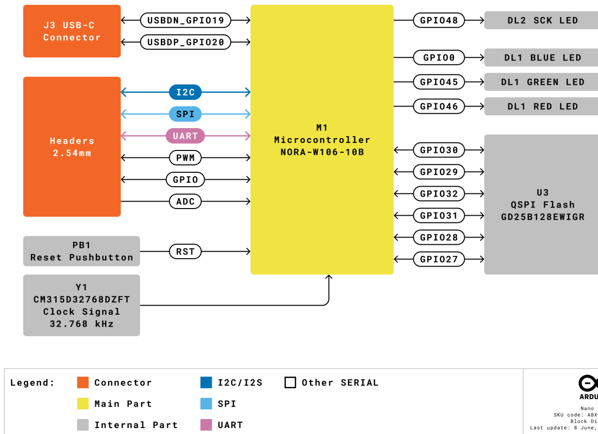
Arduino Nano ESP32 Block Diagram
